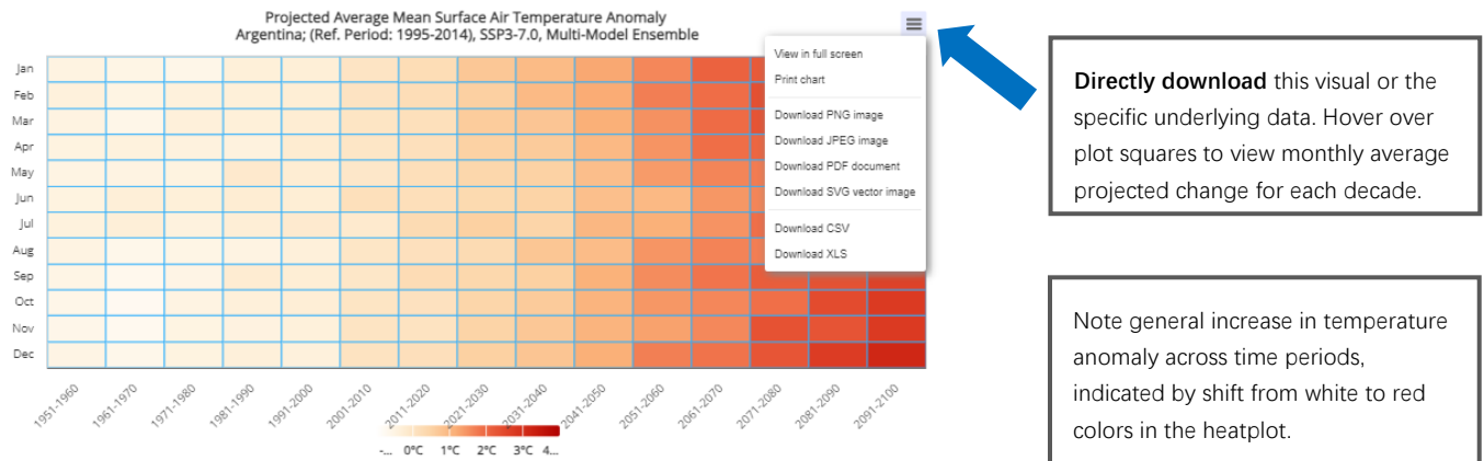
Figure O. Heatplot of Mean Average Temperature Anomaly Projections for Argentina. Note that a heatplot represents anomalies calculated against the historical reference period. Thus, it is feasible to see negative values for earlier time periods (i.e., 1950s, 1960s, etc.) in the heatplot.
