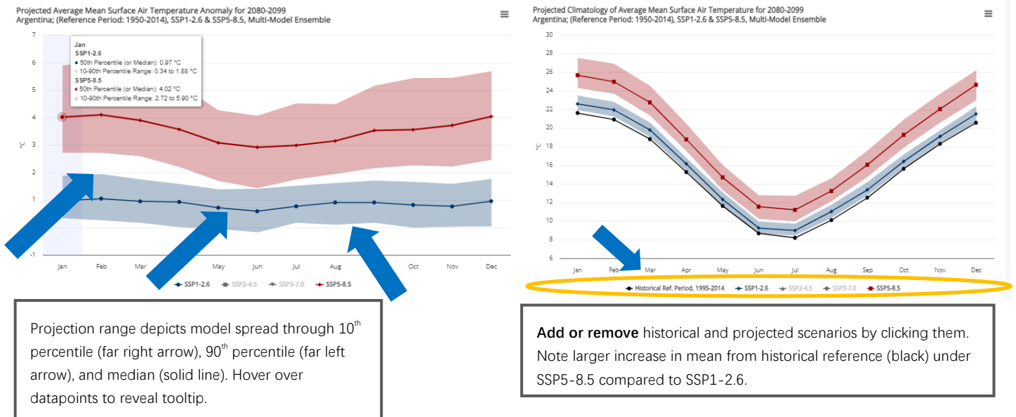
Figure N. Projected Time Series of Multi-model Ensemble for Selected Variable
