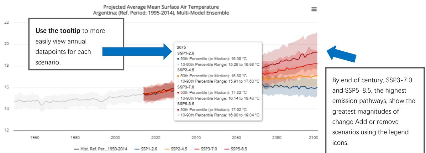
Figure N. Projected Time Series of Multi-model Ensemble for Selected Variable
