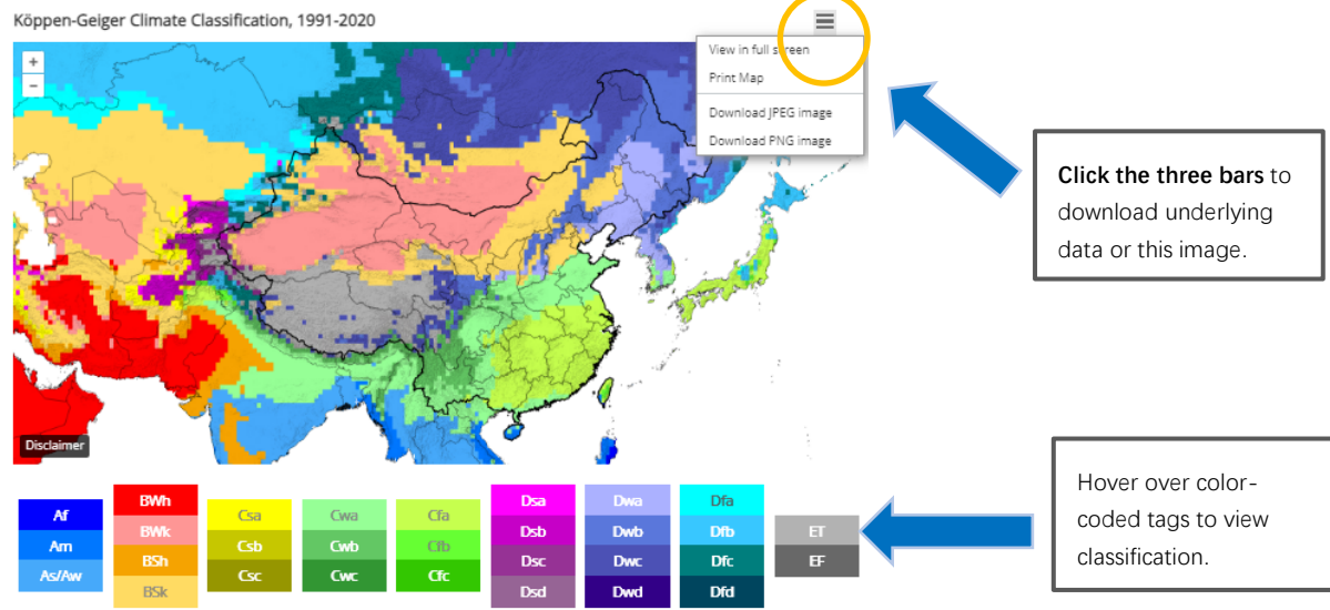
Figure A. Köppen-Geiger Climate Classification, 1991-2020 for China
